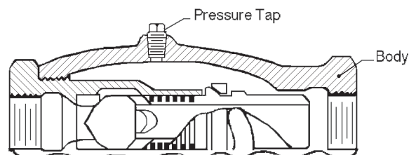
Figure 3: Opt-26 Pressure Tap, Metal Seat
