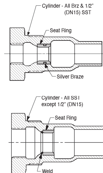
Figure 2: Opt-14 Integral Seat
